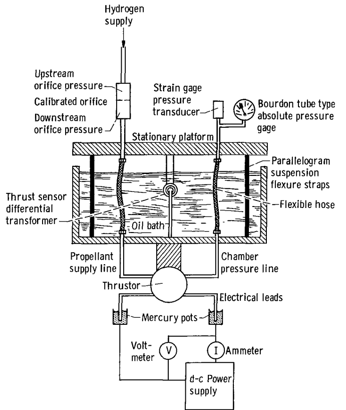
Figure 6. - Schematic drawing of thrust stand and instrumentation.
