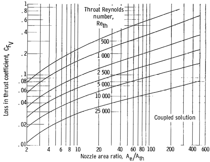
Figure 3. - Loss in thrust coefficient due to viscous effects as given by laminar-flow flat-plate theory. Stagnation temperature, 530^{\circ}\text{R} ; wall-to stagnation-temperature ratio, 1.0; nozzle divergence angle, 20^{\circ} .
