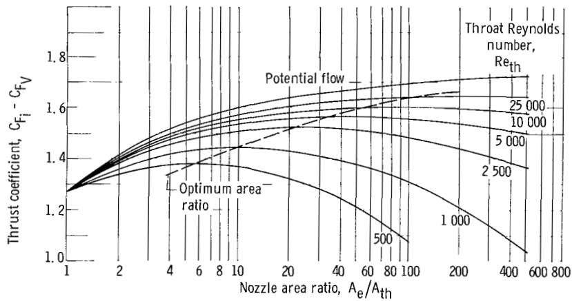
Figure 4. - Thrust coefficient including viscous losses as given by laminar-flow flat-plate theory. Stagnation temperature, 530^{\circ}\text{R} ; wall-to stagnation-temperature ratio, 1.0; nozzle divergence angle, 20^{\circ} .
